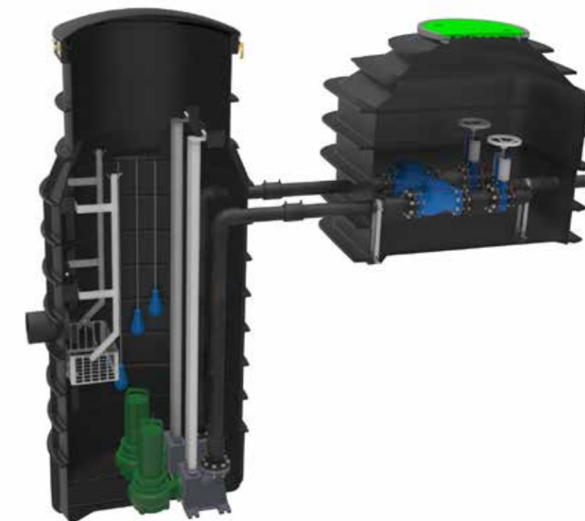
Station de relevage 1200
